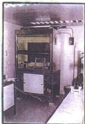
STAINLESS STEEL FUME CABINET WITH HEPA FILTER ARRANGEMENT
